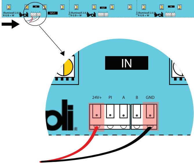
Power connection
